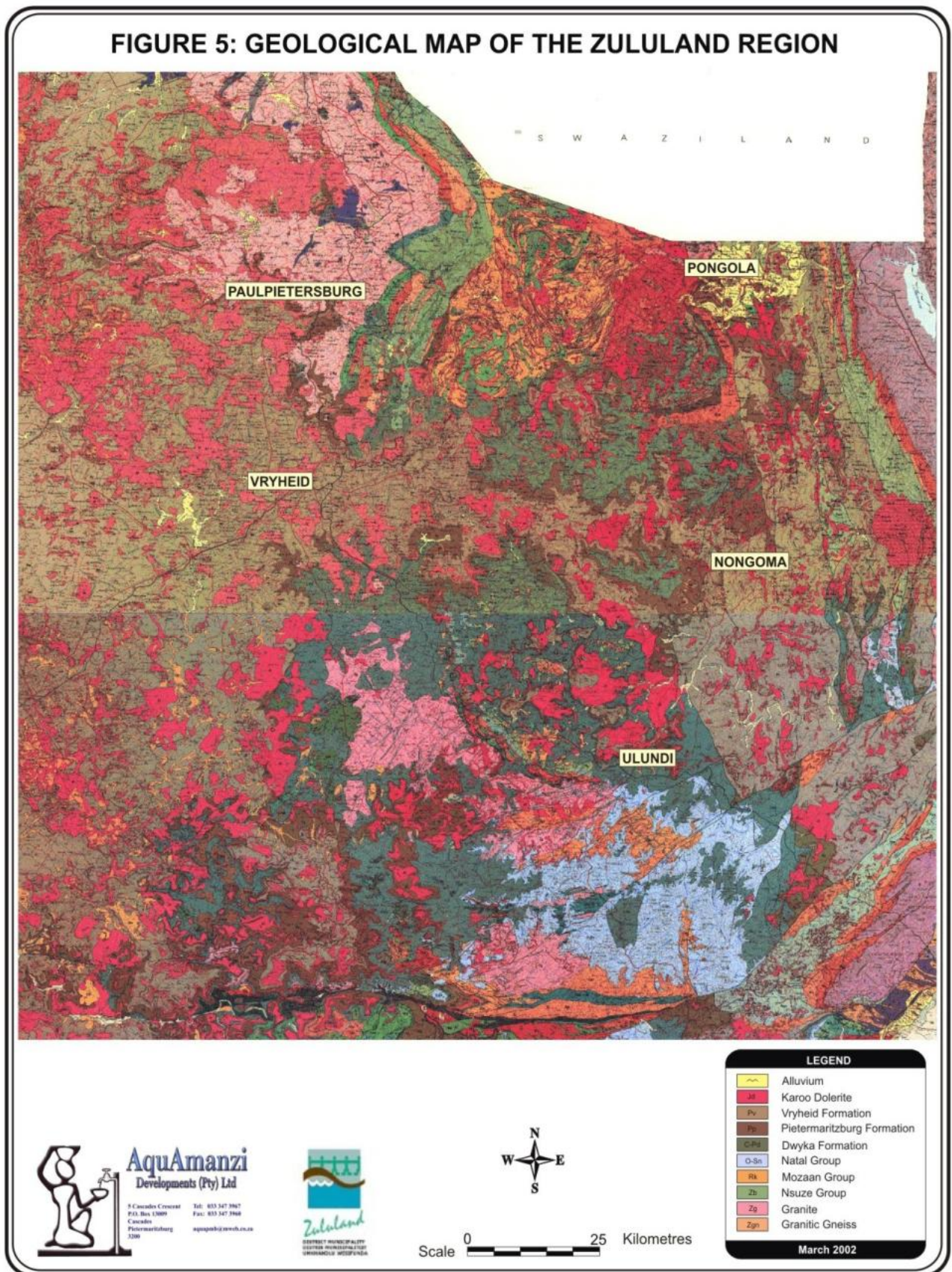
Figure 3.1: Geology of the Zululand District Municipality
